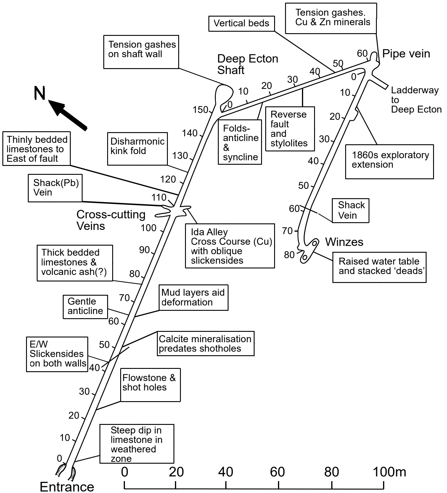
Figure C7. Ecton Mine - Salts Level. Geological Details
